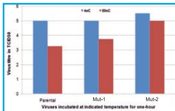
Fig 22. Thermal Inactivation kinetics of parental and mutant FMDV vaccine strains after incubating at 50°C for 1 hour.
